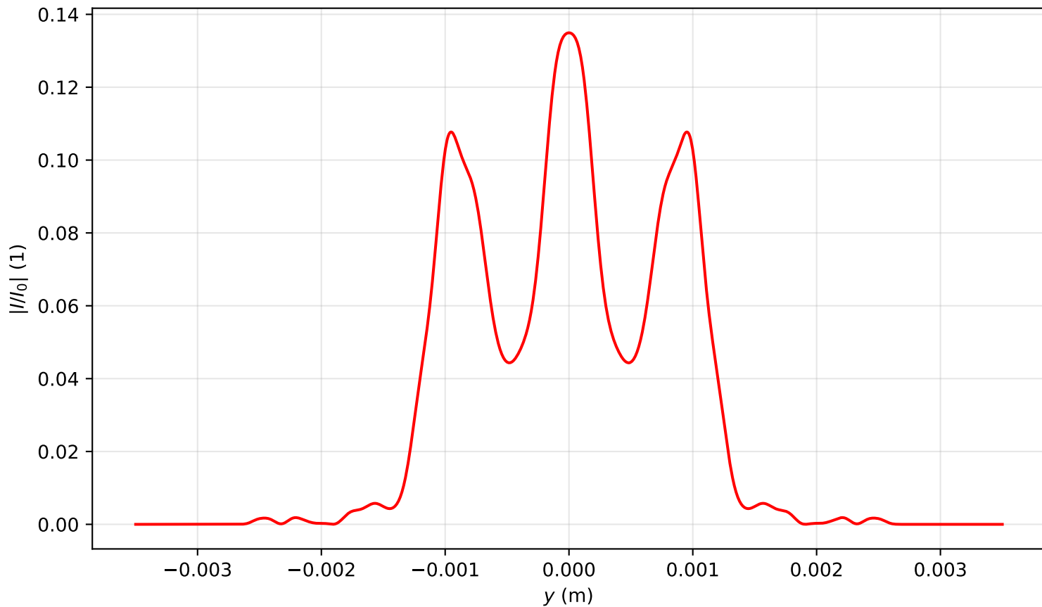
Intensity profile I(x=0, y, z=2.388)/I_0 , \text{Pin}=6.5\text{Pcr} , artificial time
